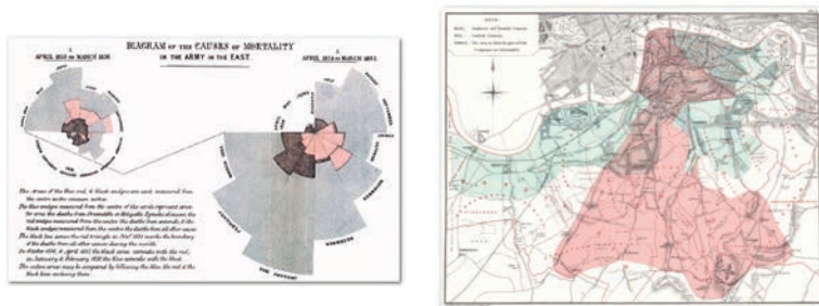
Figure 3: Snownight
