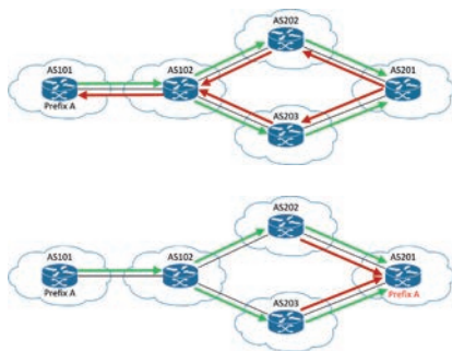
Figure 3: Prefix hijack
