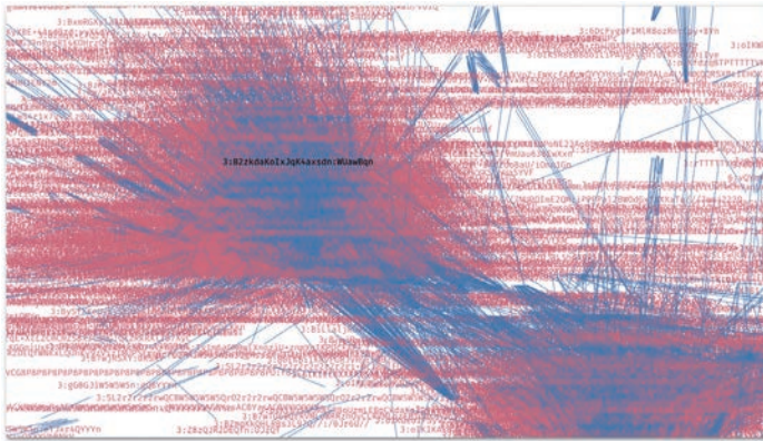
Figure 5: Left cluster
