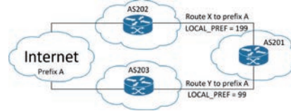
Figure 1: Route selection
