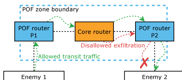
Figure 1: Which traffic originates in the POF zone, and which traffic is transit traffic, originating from outside the zone? POF detects the difference reliably
